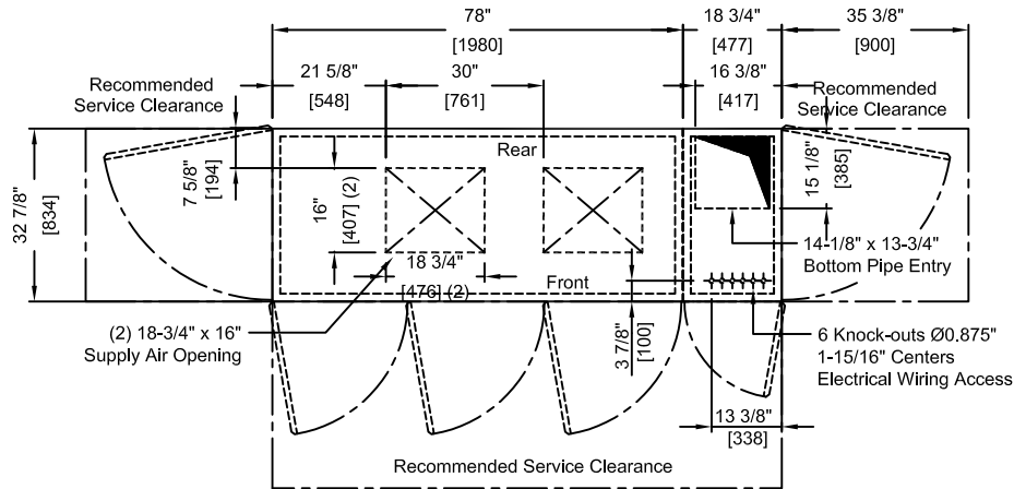
Base Frame Outline Detail - Section 'AA'
