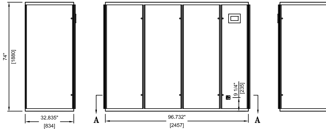
Left end view
