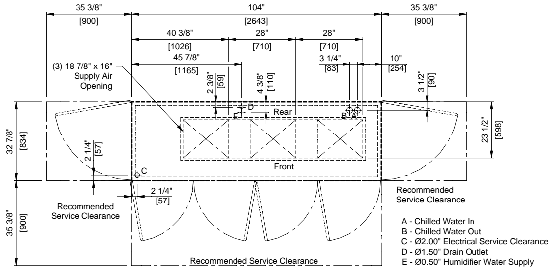
Base Frame Outline Detail - Section 'AA'
