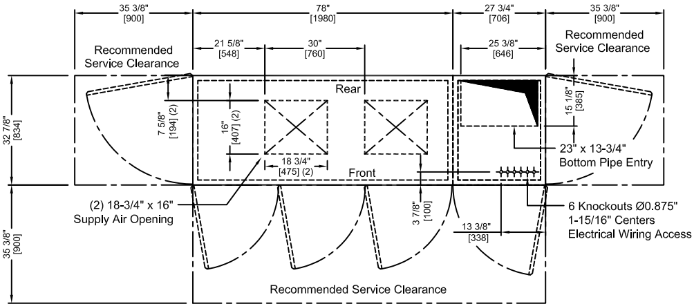
Base Frame Outline Detail - Section 'AA'
