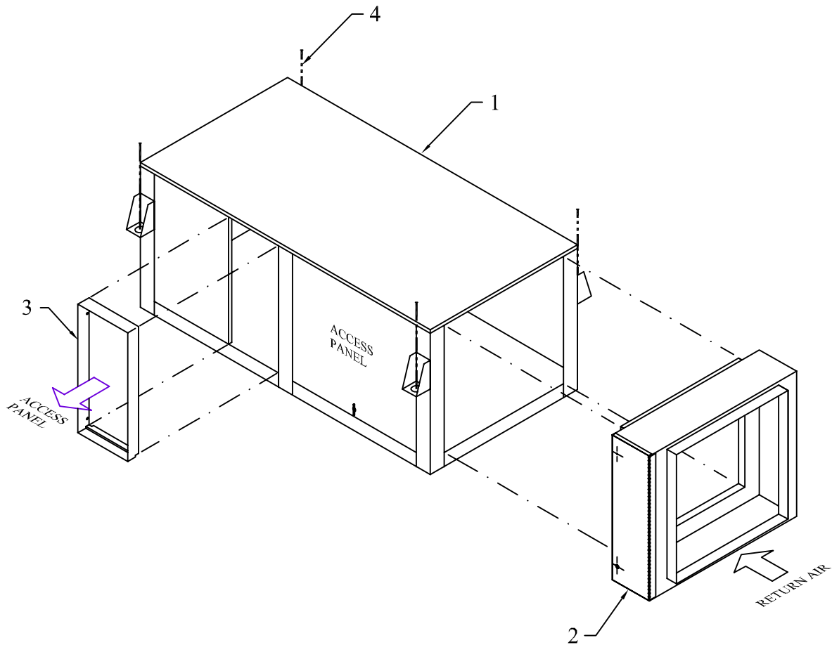
REAR VIEW
