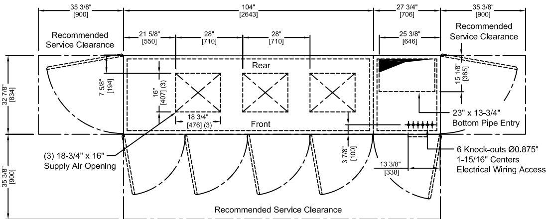
Base Frame Outline Detail - Section 'AA'
