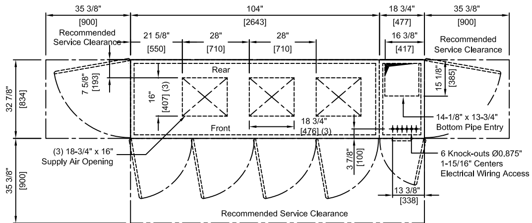
Base Frame Outline Detail - Section 'AA'
