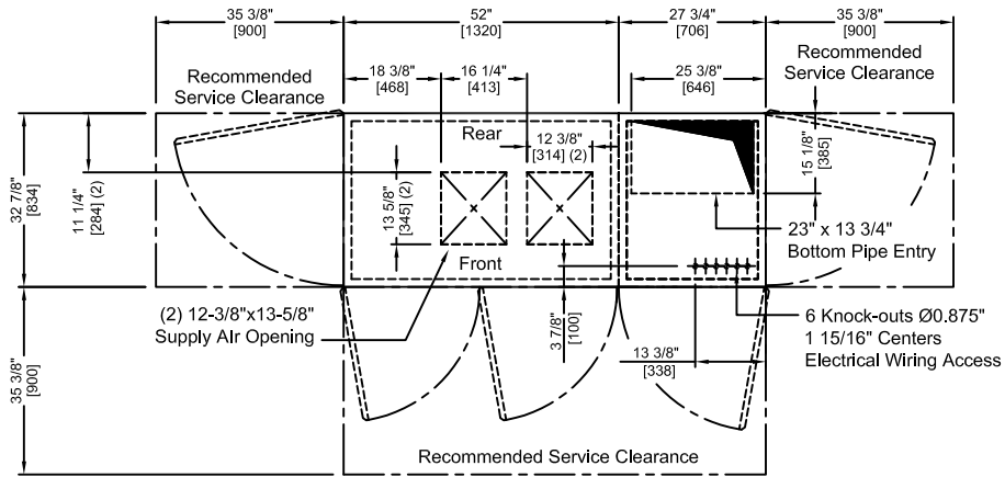
Base Frame Outline Detail - Section 'AA'
