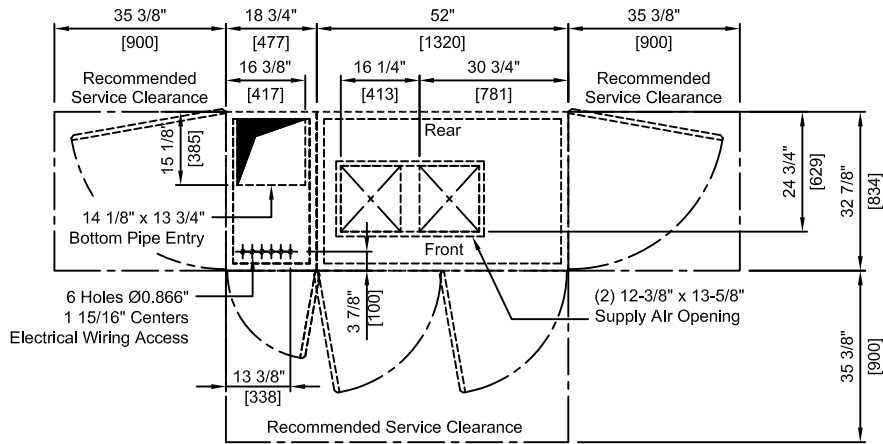
Base Frame Outline Detail - Section 'AA'
