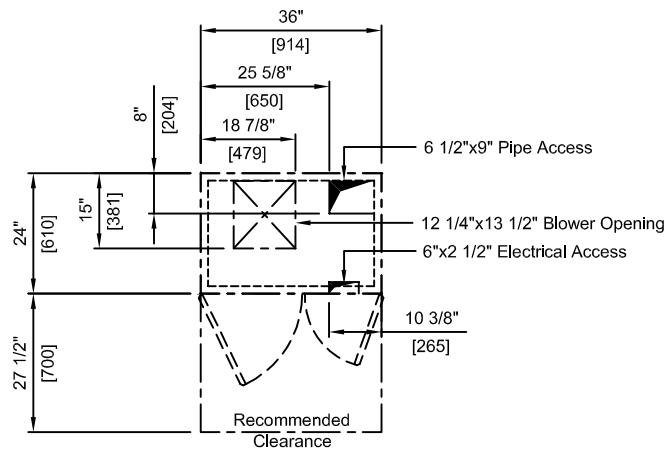
Base Frame Outline Detail - Section 'AA'
