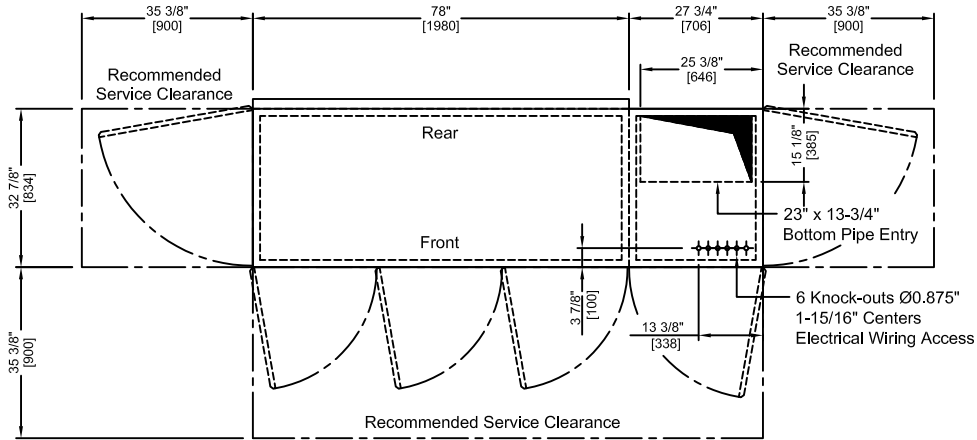
Base Frame Outline Detail - Section 'AA'
