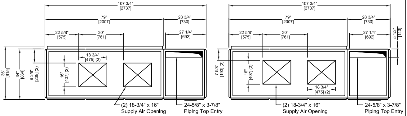
Plan (Back Discharge)
